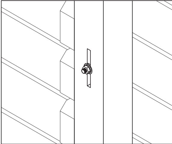
Detail in
