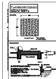
Fundamentplan
